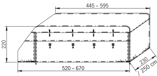
Suitable for caravans with a length of 520 to 670 cm
